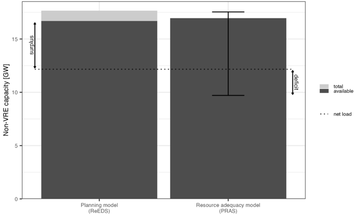
Available firm capacity in LGEE with weather from 7:00 AM Dec 12, 2012
